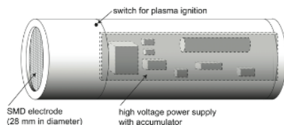
Figure 2. Schematic image of the miniFlatPlaSter plasma device.
