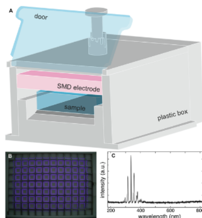
Figure 1. Schematic image of the FlatPlaSter plasma device.
